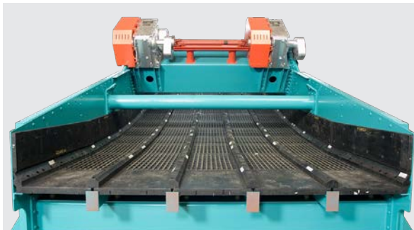
Schenck Process Banana Linear Screen
